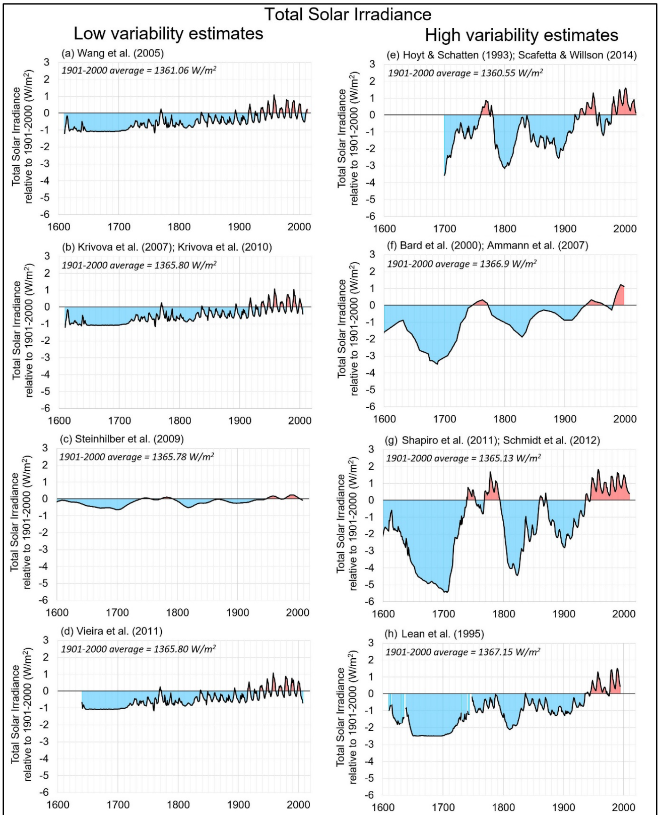
Eight different estimates of how TSI has changed since the 17 th century relative to the 20 th century average (1901-2000). All estimates are calibrated to match with one of the satellite based TSI composites over the satellite era and then each uses different “solar proxies” to describe the trends before the satellite era. (Adapted from Soon, Connolly, and Connolly, 2015)
