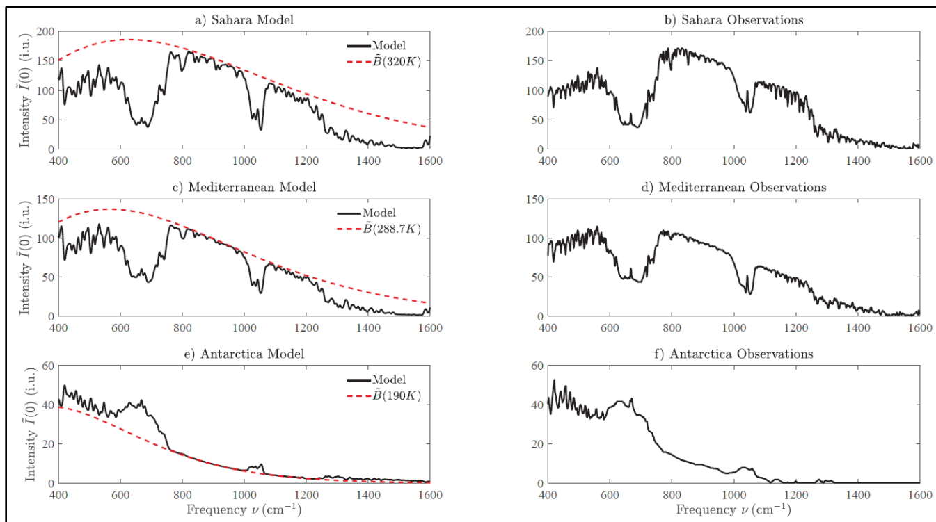
Thermal radiation intensities at the top of the atmosphere observed with a Michaelson interferometer in a satellite 4 (right) and theoretically modelled intensities 5 (left). Three latitudes are shown: The Sahara Desert, the Mediterranean Sea, and Antarctica. The intensity unit is 1 i.u. = 1 mW m -2 cm sr -1 . Radiative forcing is negative over wintertime Antarctica since the relatively warm greenhouse gases in the troposphere – mostly carbon dioxide, ozone, and water – radiate more to space than the cold ice surface, at a temperature of T = -117.4^{\circ}\text{F} (-83^{\circ}\text{C}) , could radiate through a transparent atmosphere.
