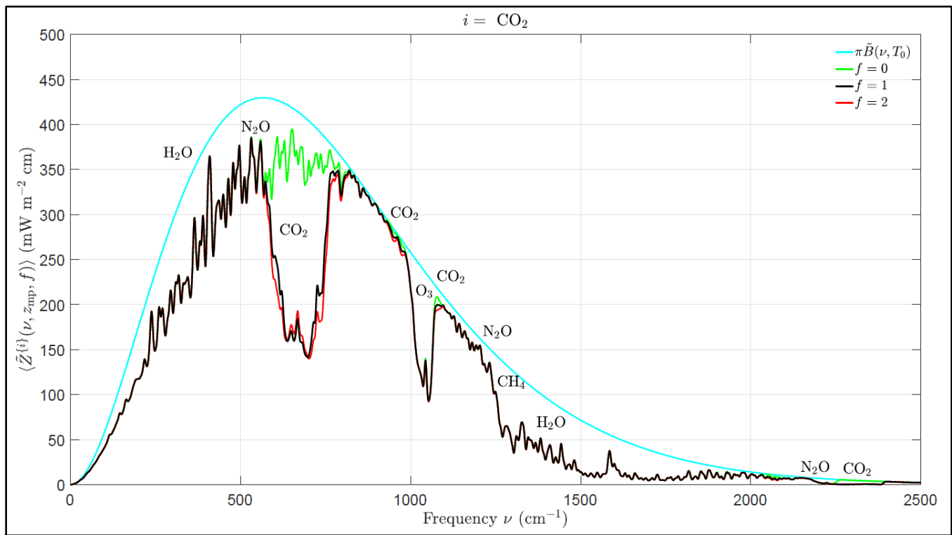
The spectral forcing at current levels of carbon dioxide, CO2 (the black curve with f = 1 ), or if concentrations of carbon dioxide are doubled (the red curve with f = 2 ), or if all carbon dioxide is removed (the green curve with f = 0 ).
